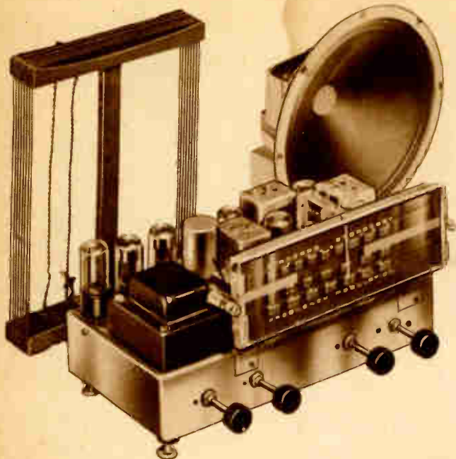
Model 1-1100. —Operates on 105-125 volts AC, 50/60 cycles. Shipping weight 20 pounds. Chassis size: 13 \frac{3}{4} " long, 9" deep, 8 \frac{7}{8} " high. $89.50 Your Cost
